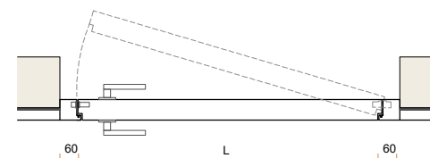
Porta a spingere Door by pushing
